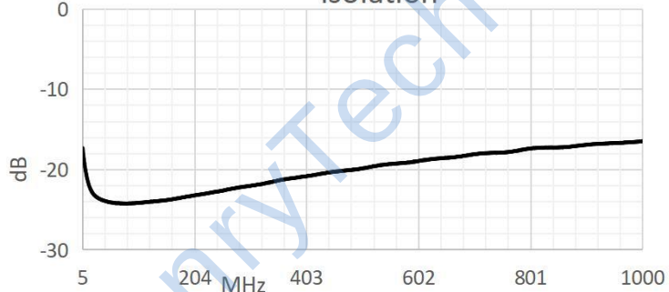
Isolation
