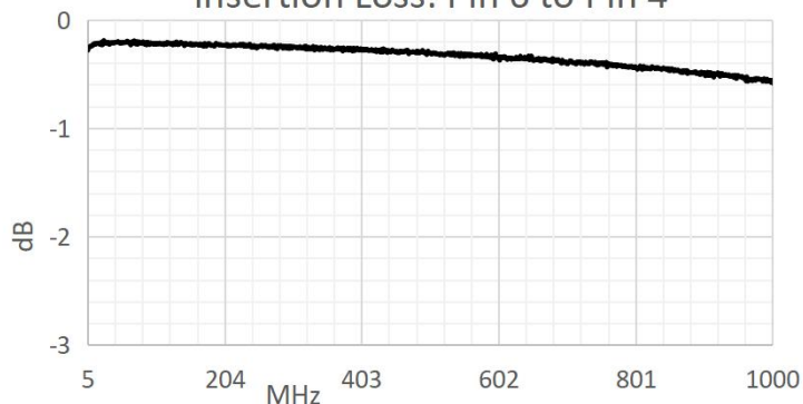
Insertion Loss: Pin 6 to Pin 4
